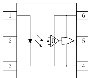
Pin Configuration
