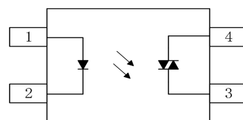
Pin Configuration
