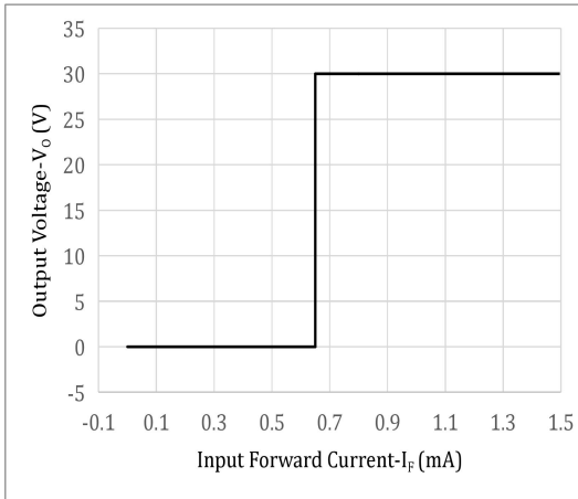
Fig.15 Output Voltage vs. Input Forward Current
