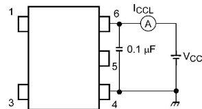
Fig22. I_{CCL} Test Circuit
