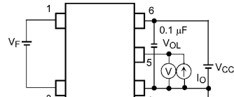
Fig20. V_{OL} Test Circuit
